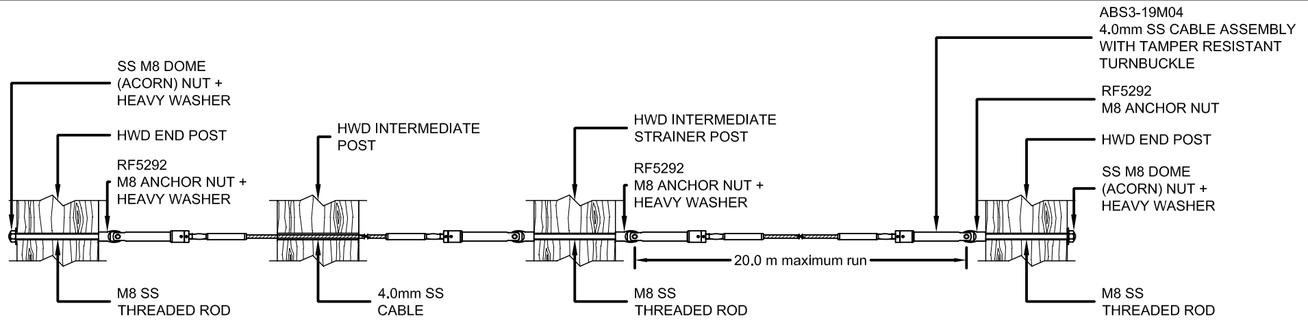
ELEVATION ○ OSA-2 RONSTAN BALUSTRADE SYSTEM
