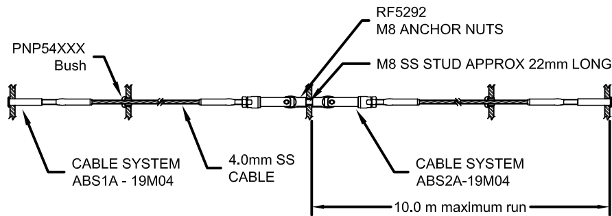
ELEVATION ○ OSA-1 RONSTAN BALUSTRADE SYSTEM
