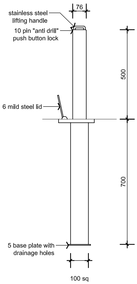
Rhino Telescopic Security Bollard RT/RD4 from Outdoor structures Australia
