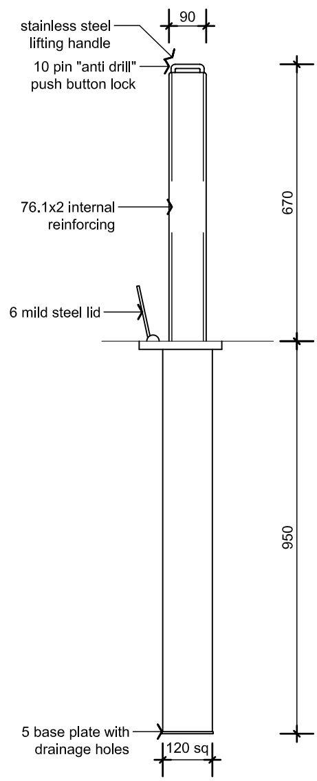
Rhino Telescopic Security Bollard RT/R8 from Outdoor structures Australia
