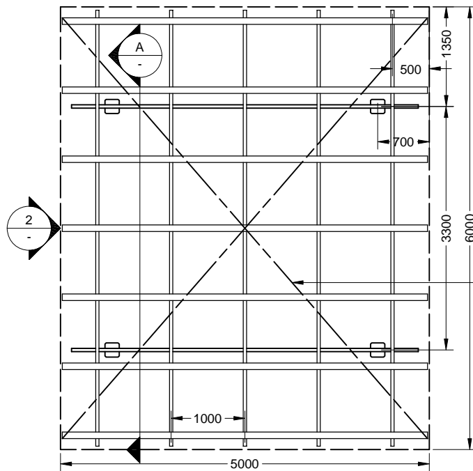
PLAN ROOF FRAMING Scale: 1:50
