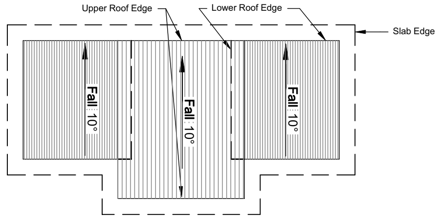
PLAN 1/1 ROOF Scale: 1:100
